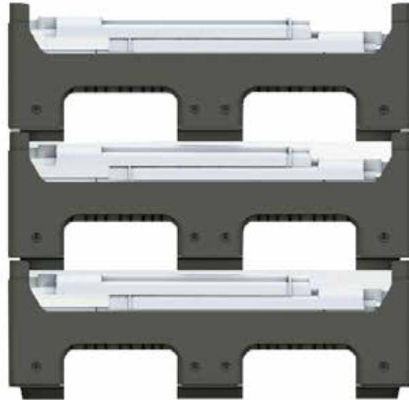
345 mm Single Folding Height 315 mm Stacking Folding Height
